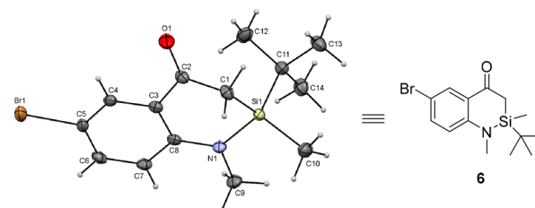
Figure 2. Molecular structure of 6 . Thermal ellipsoids are set at 50% probability level. Selected bond distances (Å) and angles (deg): N1–Si1 1.746, C1–Si1 1.859, N1–Si1–C1 101.29, O–C2–C3–C4 21.94.
