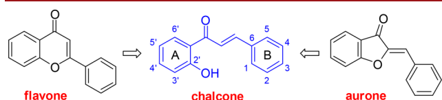
Figure 1. Chalcone as a precursor in the biosynthesis of flavonoids.
